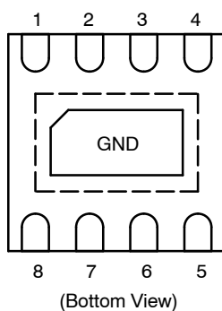
Figure 3. Pin Diagram
