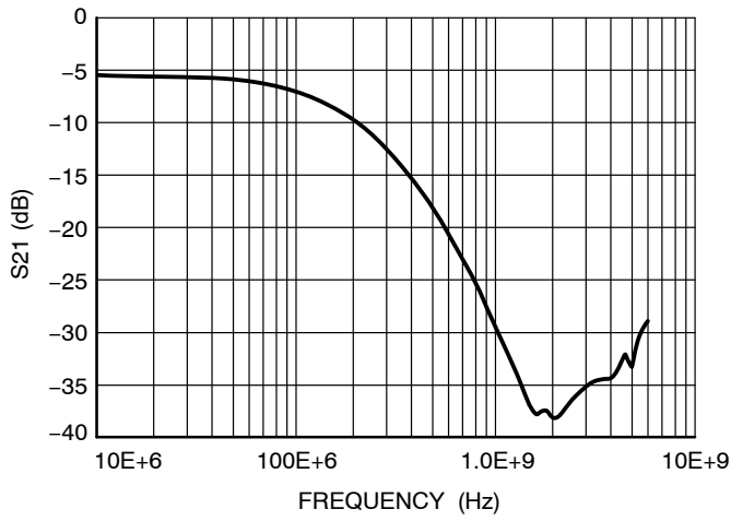
Figure 4. Typical Insertion Loss Characteristic
