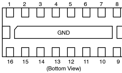
Figure 3. Pin Diagram
