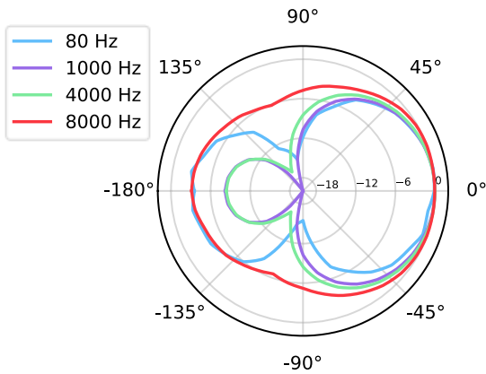
Figure 8.1: Polar pattern
