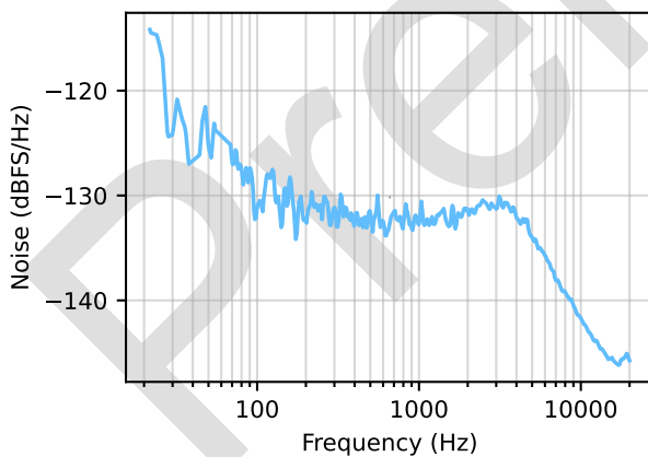
Figure 8.5: Noise floor
