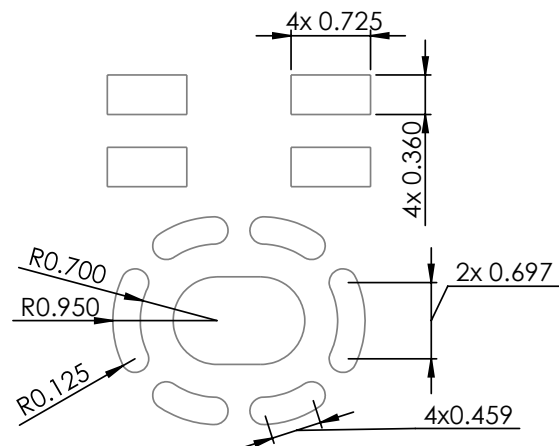
Figure 8.3 Example solder stencil pattern (mm)
