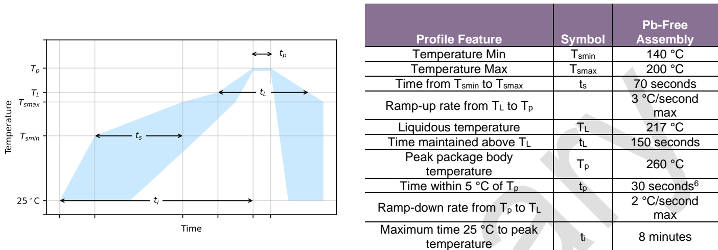
Figure 8.5: Reflow profile
