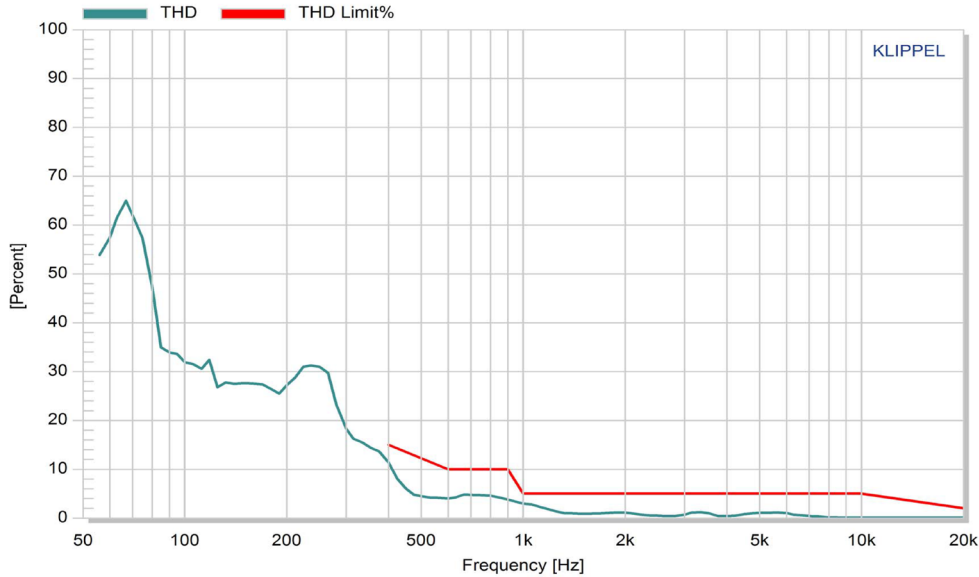
Total Harmonic Distortion Curve
