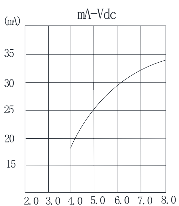
Voltage vs. Current Consumption at 25°C
