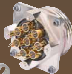
D38999 Series III Connectors (standoff shell at right and standard shell below) with Quadrax PC Tail Contacts
