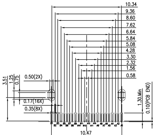
RECOMMENDED P.C.B LAYOUT TOP VIEW TOLERANCES \pm 0.05\text{MM}
