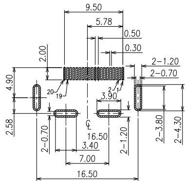
RECOMMENDED PCB LAYOUT TOLERANCE: ±0.05mm
