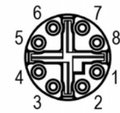
M12 Pin assignment
