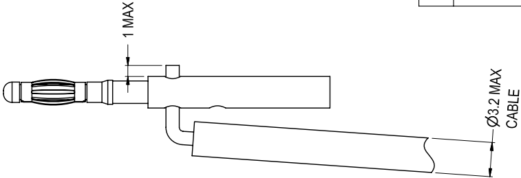
VIEW SHOWING SOLDER CONNECTION OF CABLE TO CONTACT
