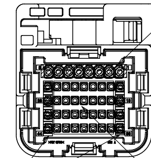
FIG.1 APPLICABLE WIRE SIZE AND CAVITY SETTING 適用電線サイズとキャビティ設定
