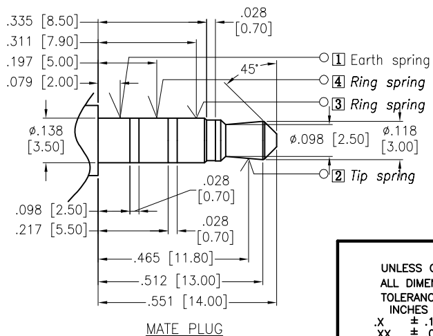
MATE PLUG
