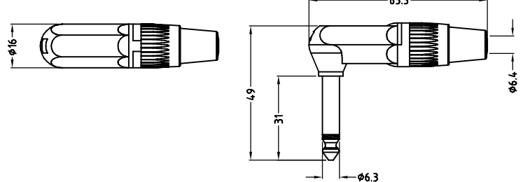
SEP/1C Professional 1/4" mono screened right angle Jack Plug. Metal body with black plastic cover. Stereo version SEP/3C also available. Rivetted construction.
