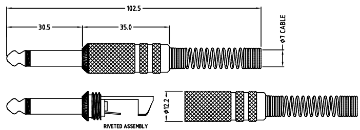
P1C 1/4" screened Jack Plug. Metal body. Rivetted construction
