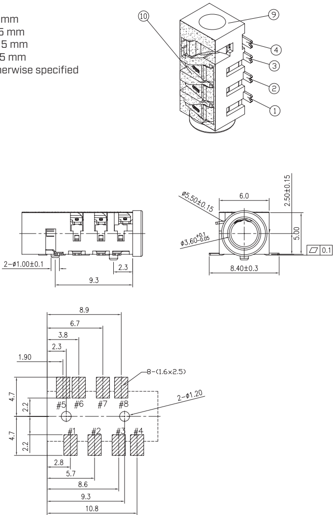
Recommended PCB Layout Top View
