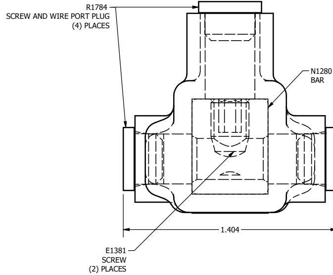
VIEW A-A SCALE 2.5:1
