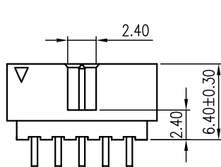
4-12 POSTIONS PROFILE
