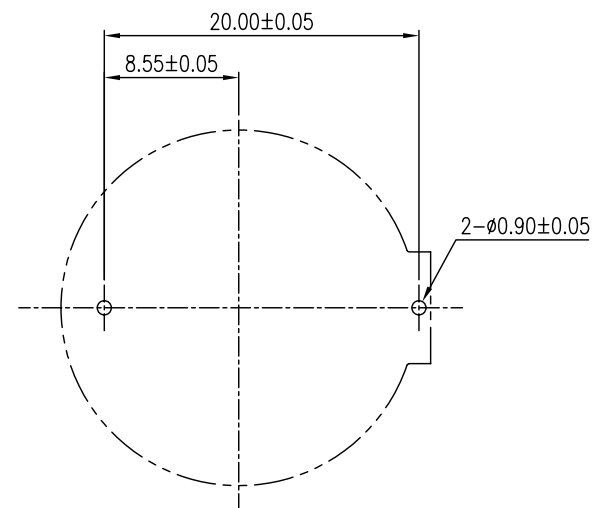
RECOMMENDER PCB LAYOUT
