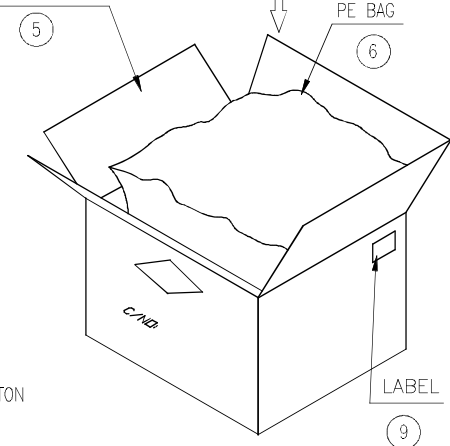
OUTER CARTON
