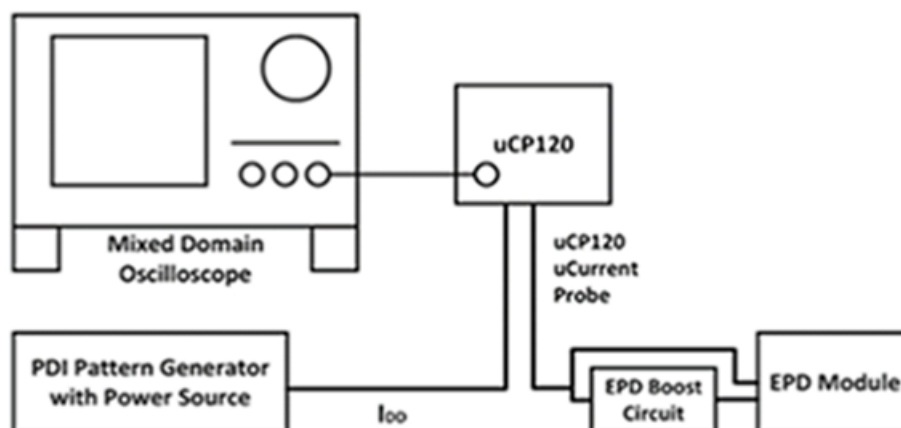
Figure 3-3 Current Measurement
