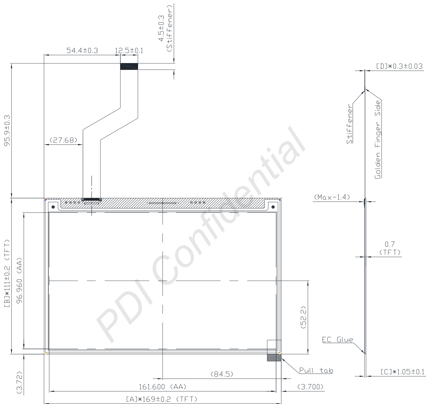
Figure 1-1 EPD Drawing
