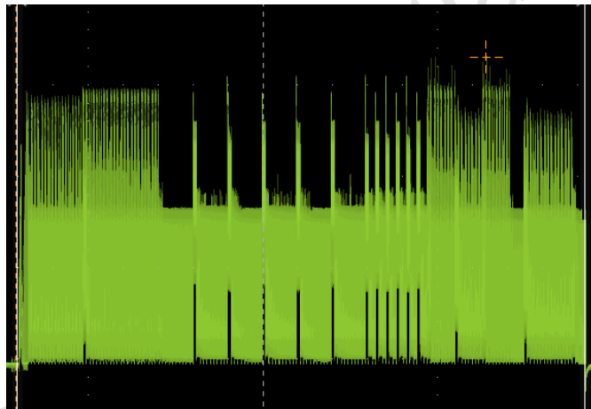
Figure 3-2 Image Update Current Profile
