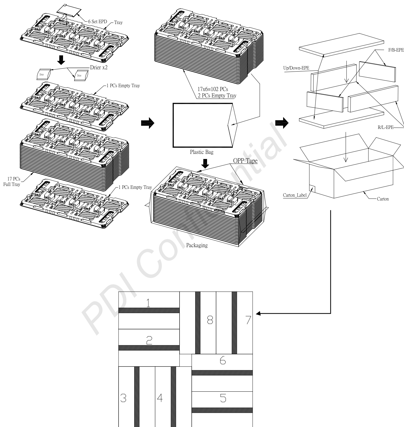
Figure 7-1 Packing Diagram
