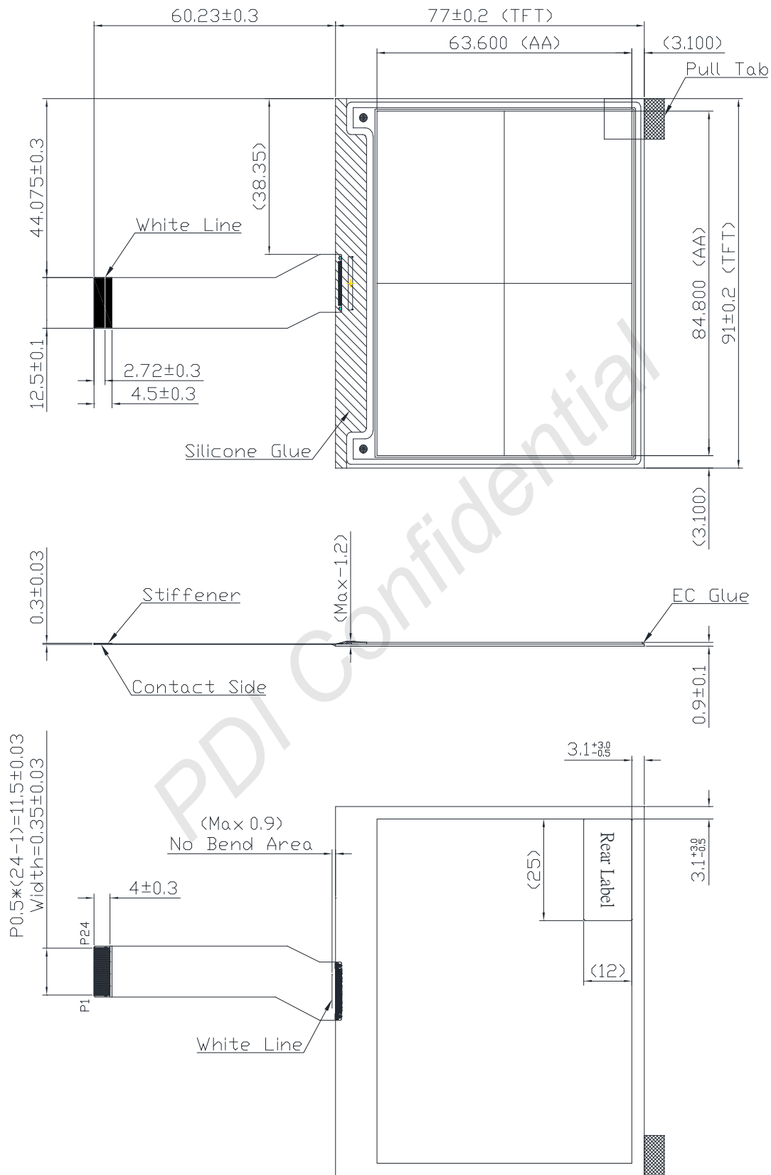
Figure 1-1 EPD Drawing
