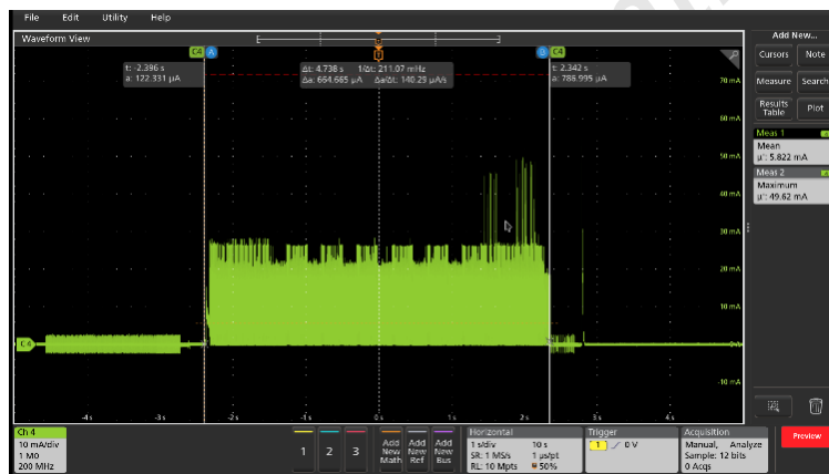
Figure 3-2 Image Update Current Profile
