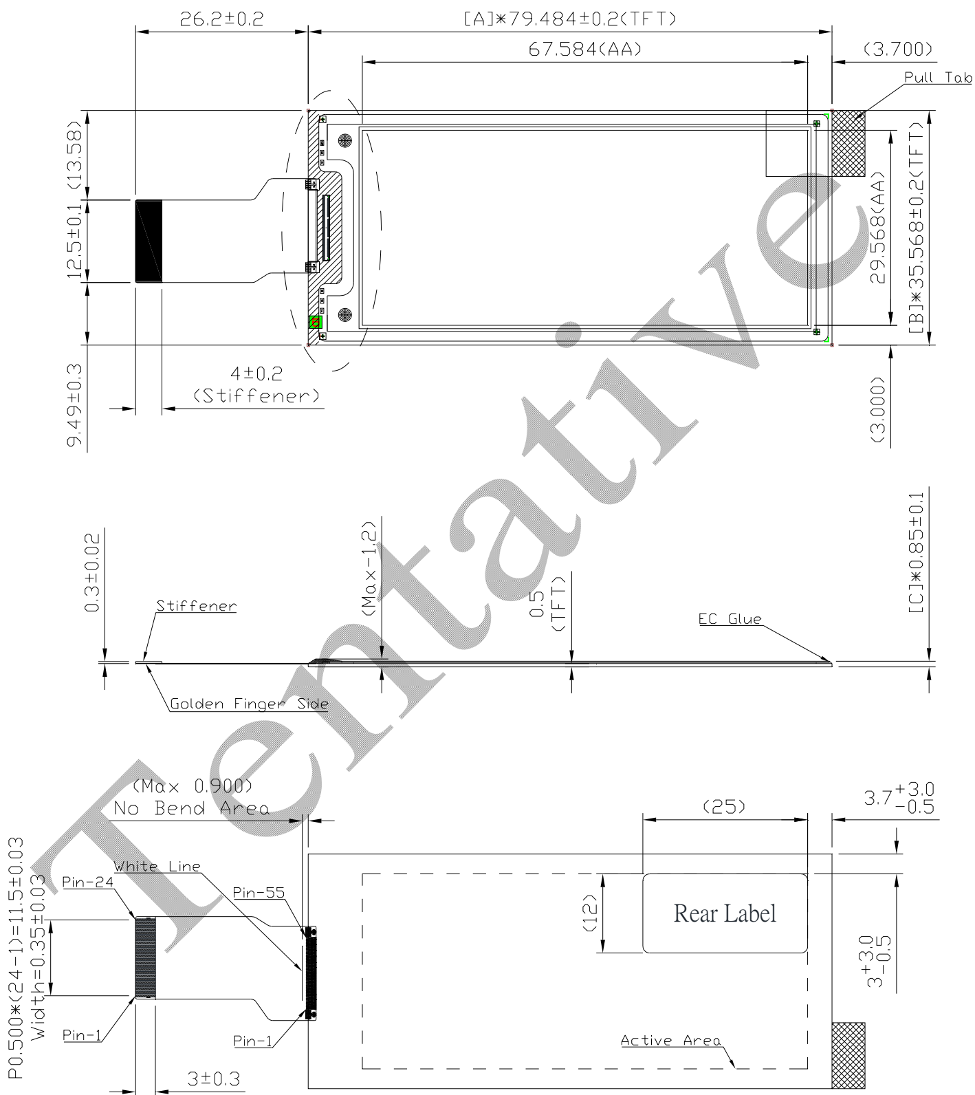
Figure 1-1 EPD Drawing
