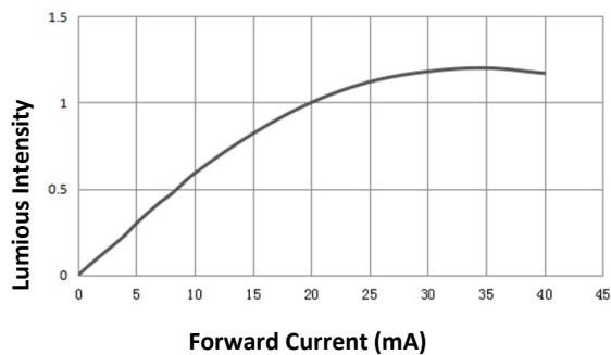
Luminous Intensity vs. Forward Current
