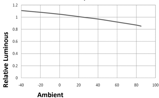
Luminous Intensity vs. Ambient Temperature
