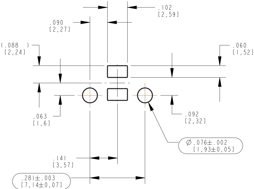
SOLDER PAD/HOLE LAYOUT FOR SINGLE COLOR SCALE 4.000
