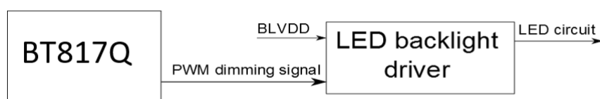
Figure 10. Backlight driver block diagram
