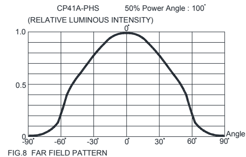
FIG.8 FAR FIELD PATTERN
