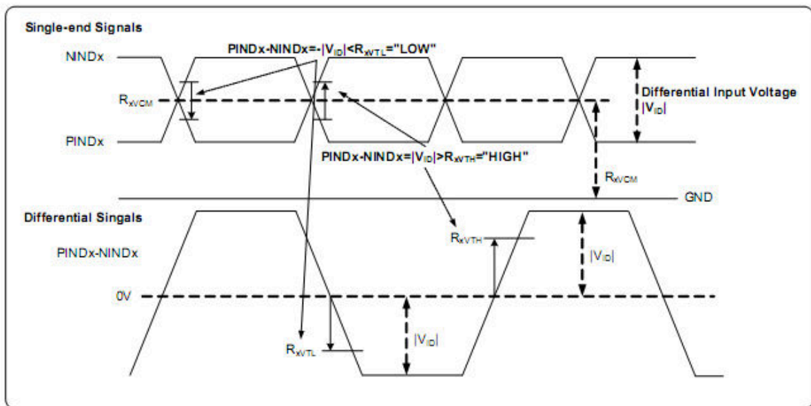
Single-end signals
