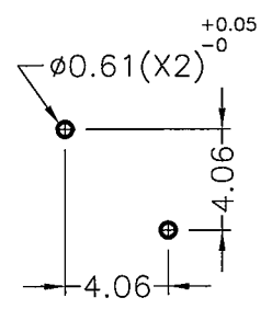
MOUNTING HOLE
