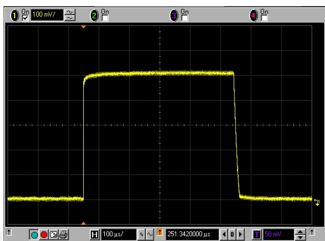
vertical 10 A/div, horizontal 100 μs/div pulse: 500 μs@50 A
