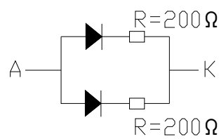
Curcuit Diagram
