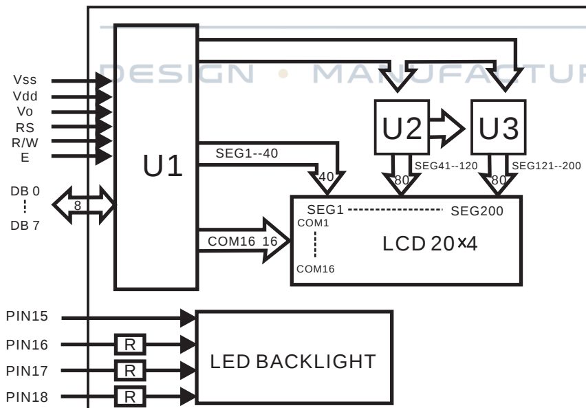
BLOCK DIAGRAM
