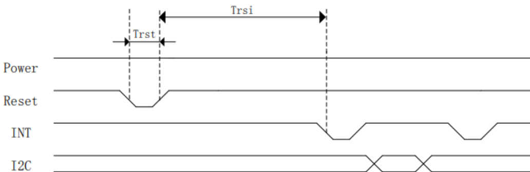
Figure 3-6 Reset Sequence
