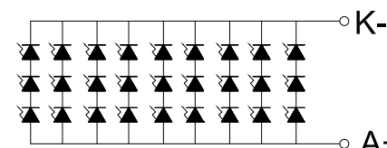
LED CIRCUIT
