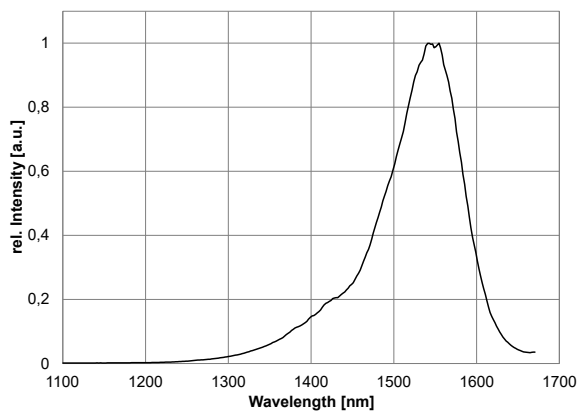
Optical Spectrum
