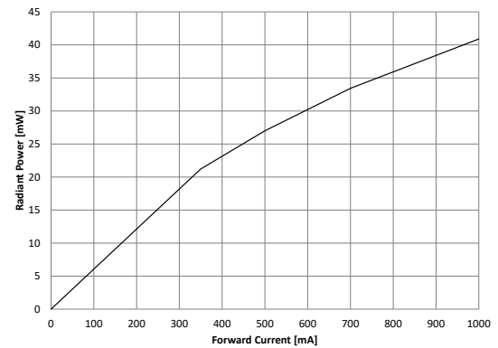
Intensity vs. Forward Current
