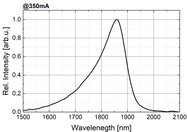
Relative Spectral Emission
