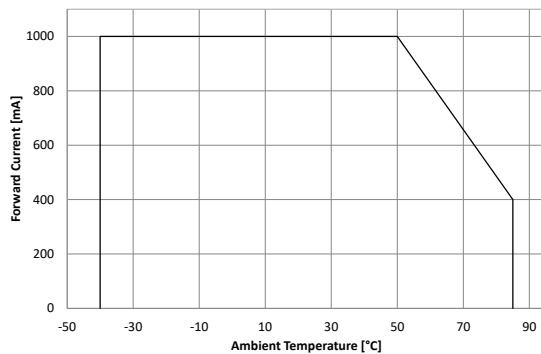
Max. Forward Current vs. Ambient Temperature
