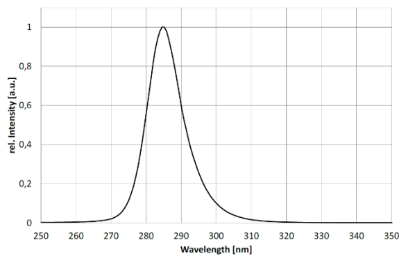
Optical Spectrum
