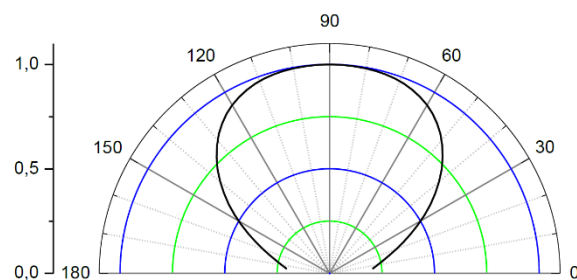
Radiation Pattern
