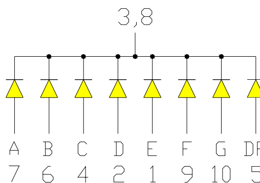
OPS-S2011 ( Common Cathode )
