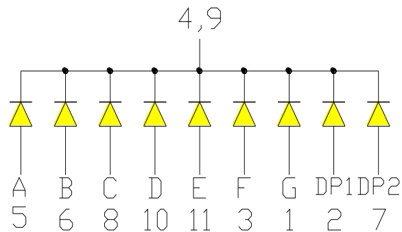
12 PIN No Connect OPS-S2811 (Common Cathode)
