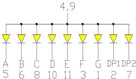
12 PIN No Connect OPS-S2812 (Common Anode)
