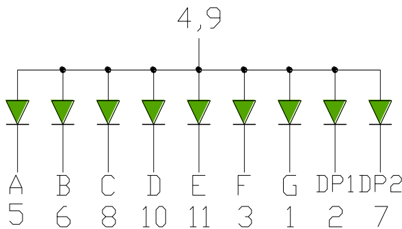
12 PIN No Connect OPS-S2812 (Common Anode)
