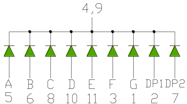
12 PIN No Connect OPS-S2811 (Common Cathode)
