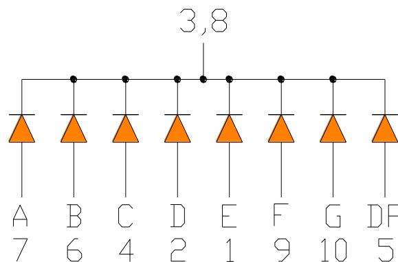
Common Cathode (OPS-S3011)
