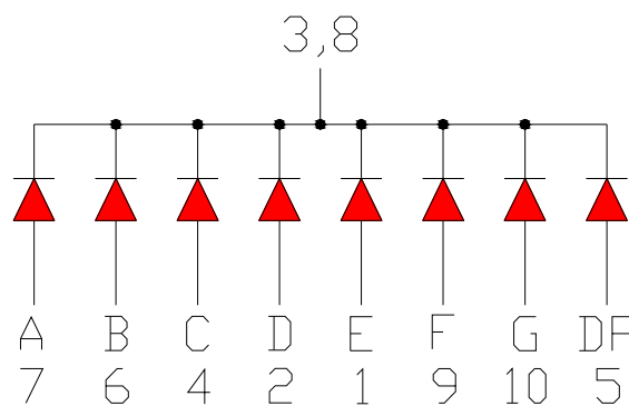
Common Cathode (OPS-S3011)
