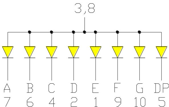
Common Anode (OPS-S3010)
