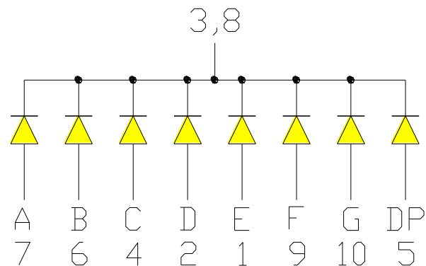
Common Cathode (OPS-S3011)
