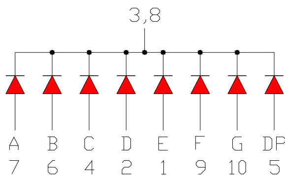
OPS-S5111 (Common Cathode)
