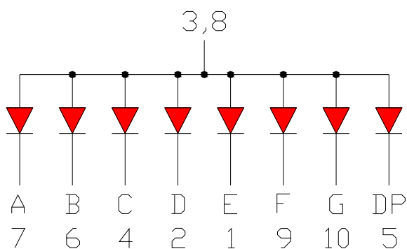
OPS-S5110 (Common Anode)
