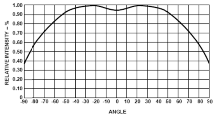
Figure 7: Radiation Pattern
