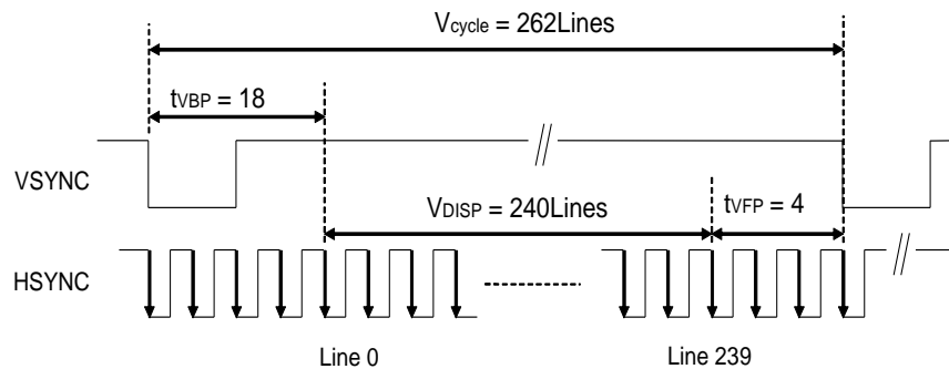
b) Vertical Data Transaction Timing
