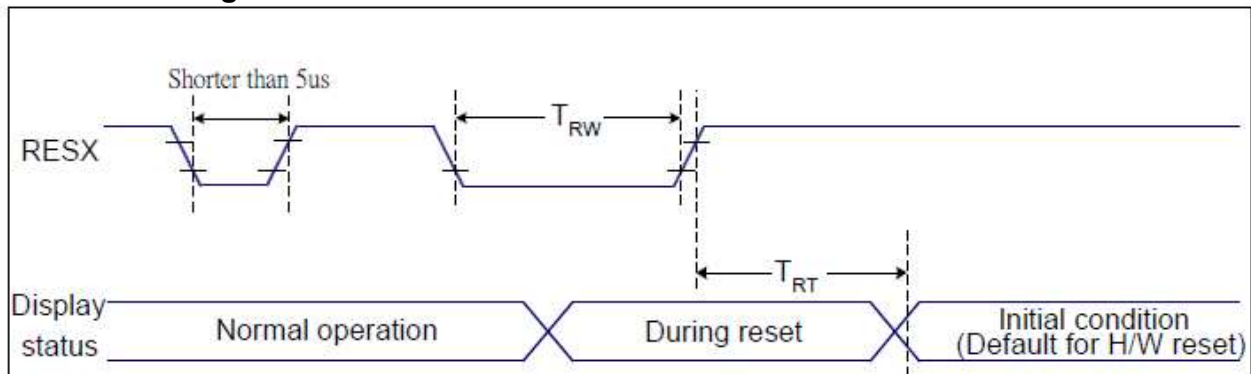
Figure 5 Reset Timing
