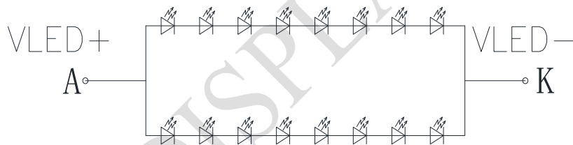
CIRCUIT DIAGRAM(8*2Dice)
