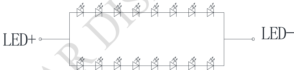
CIRCUIT DIAGRAM(8*2)
