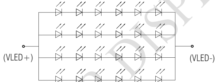
Back Light Circuit
